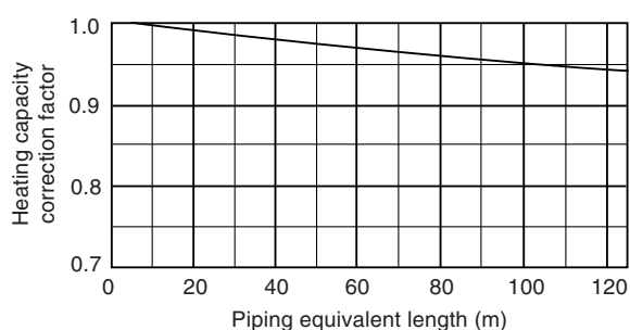
PURY-200YEMC-A
