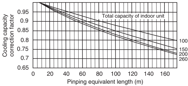
PUHY-P300YGM-A, PURY-P300YGM-A
