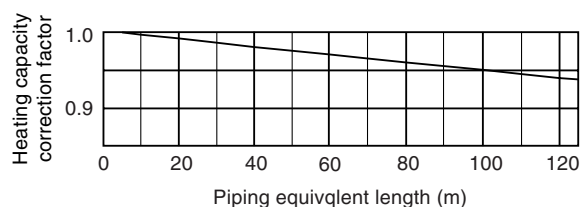
PUHY-400YEM-A/400YEMC-A PUHY-500YEM-A/500YEMC-A
