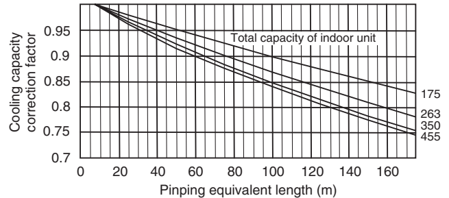
PUHY-P450YGM-A, PURY-P450YGM-A
