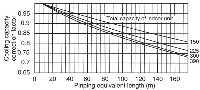
PUHY-P400YGM-A, PURY-P400YGM-A
