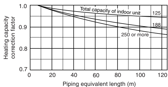
PURY-250YEMC-A
