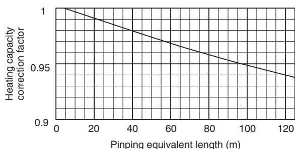
PUHY-P200YGM-A, PUHY-P250YGM-A
