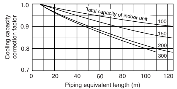
PURY-200YEMC-A
