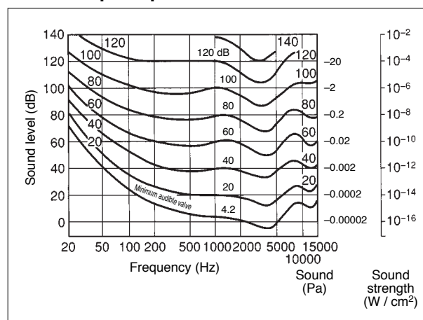
ISO audio perception curve
