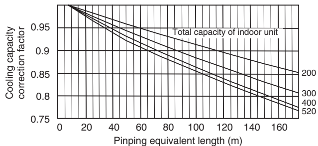
PUHY-P500YGM-A, PURY-P500YGM-A
