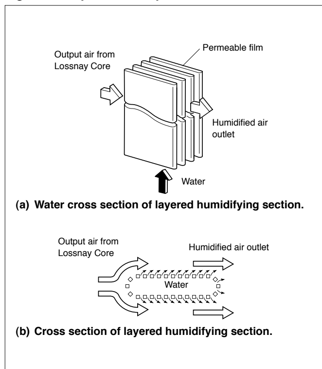
Fig. 1 Principles behind permeable film humidifier
