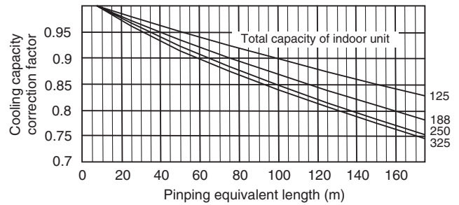
PUHY-P350YGM-A, PURY-P350YGM-A
