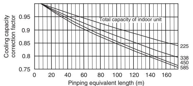
PUHY-P450YGM-A, PURY-P450YGM-A
