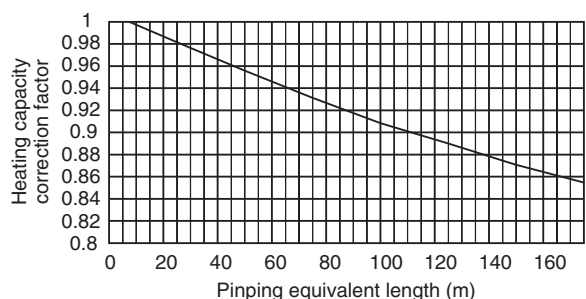
PURY-P450YGM-A, PURY-P500YGM-A
