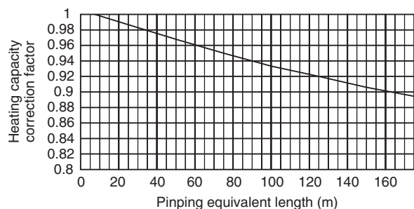
PURY-P350YGM-A, PURY-P400YGM-A
