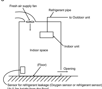
Fig.8-3. Fresh air supply upon sensor action
