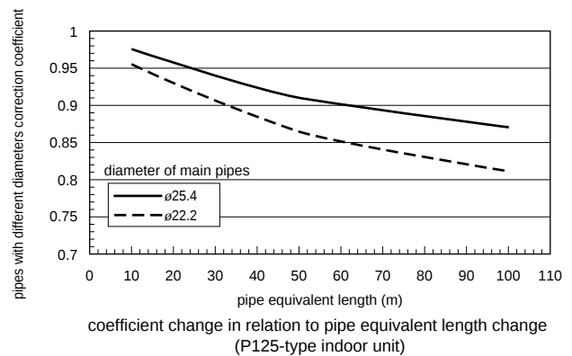
(2) Refrigerant pipe length capacity correction with P100, 125, 140-type indoor unit with the \phi 15.88\text{mm} branch pipe on the gas pipe side
