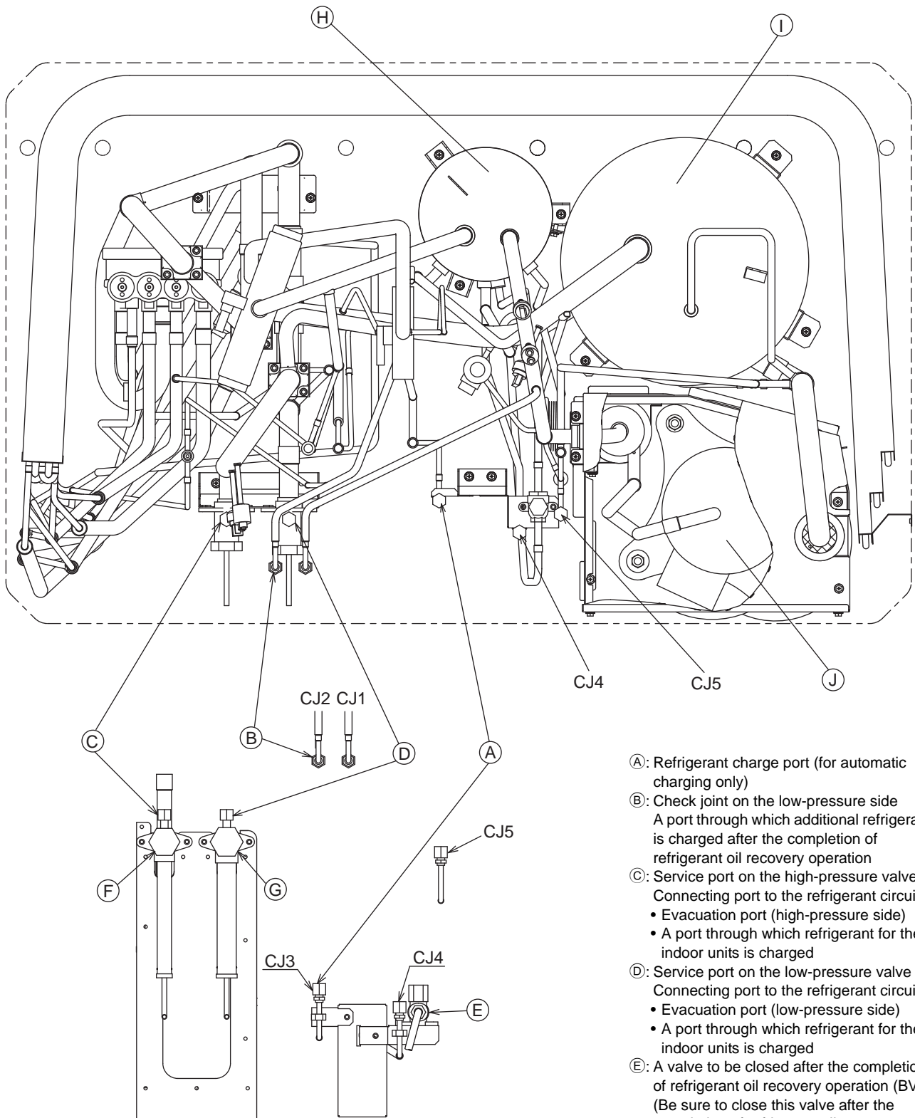
Figure 1 Top view of the refrigerant pipes inside an outdoor unit
