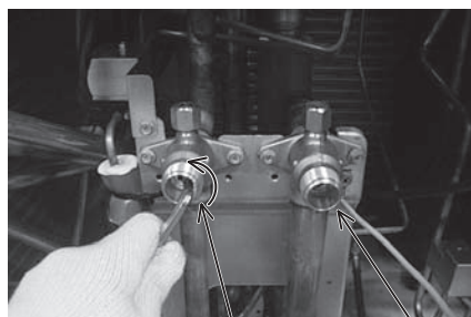
High-pressure valve
