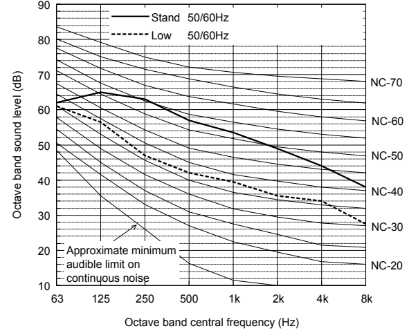
Sound level of PUHY-RP500YSJM-B(-BS)
