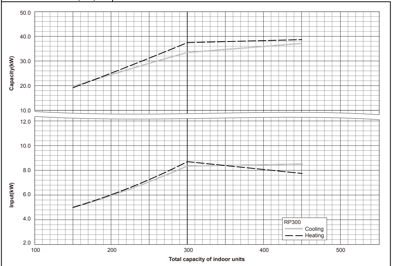
PURY-RP300YJM-B(-BS)
