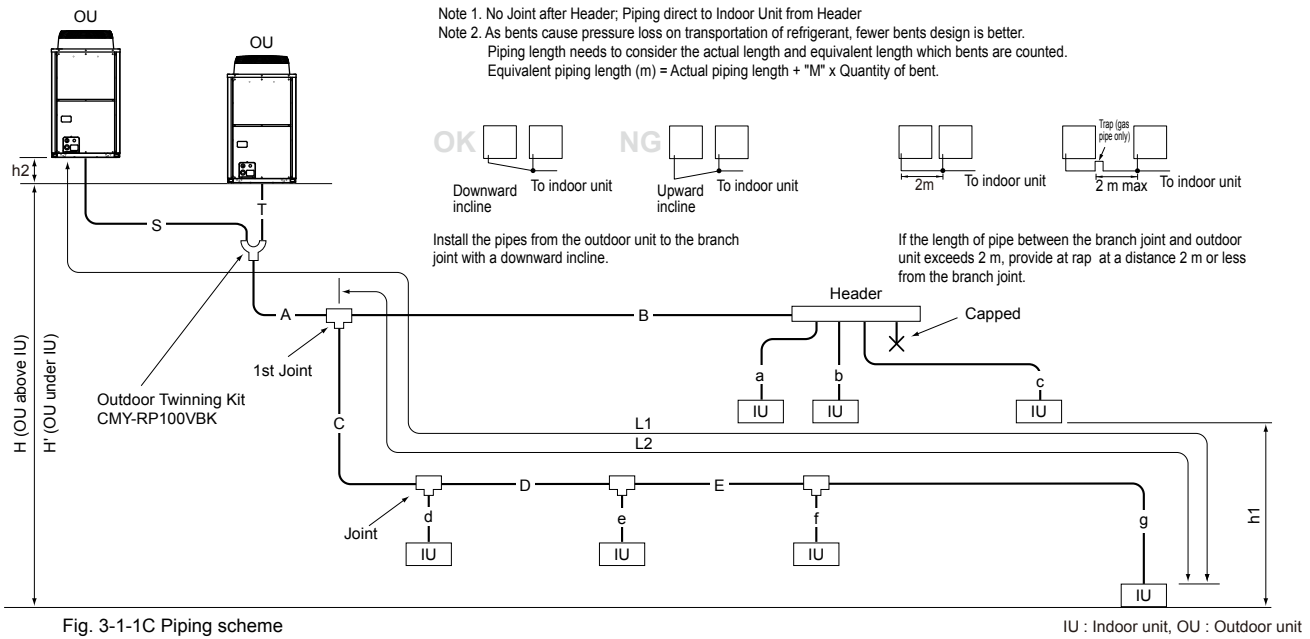
Fig. 3-1-1C Piping scheme
