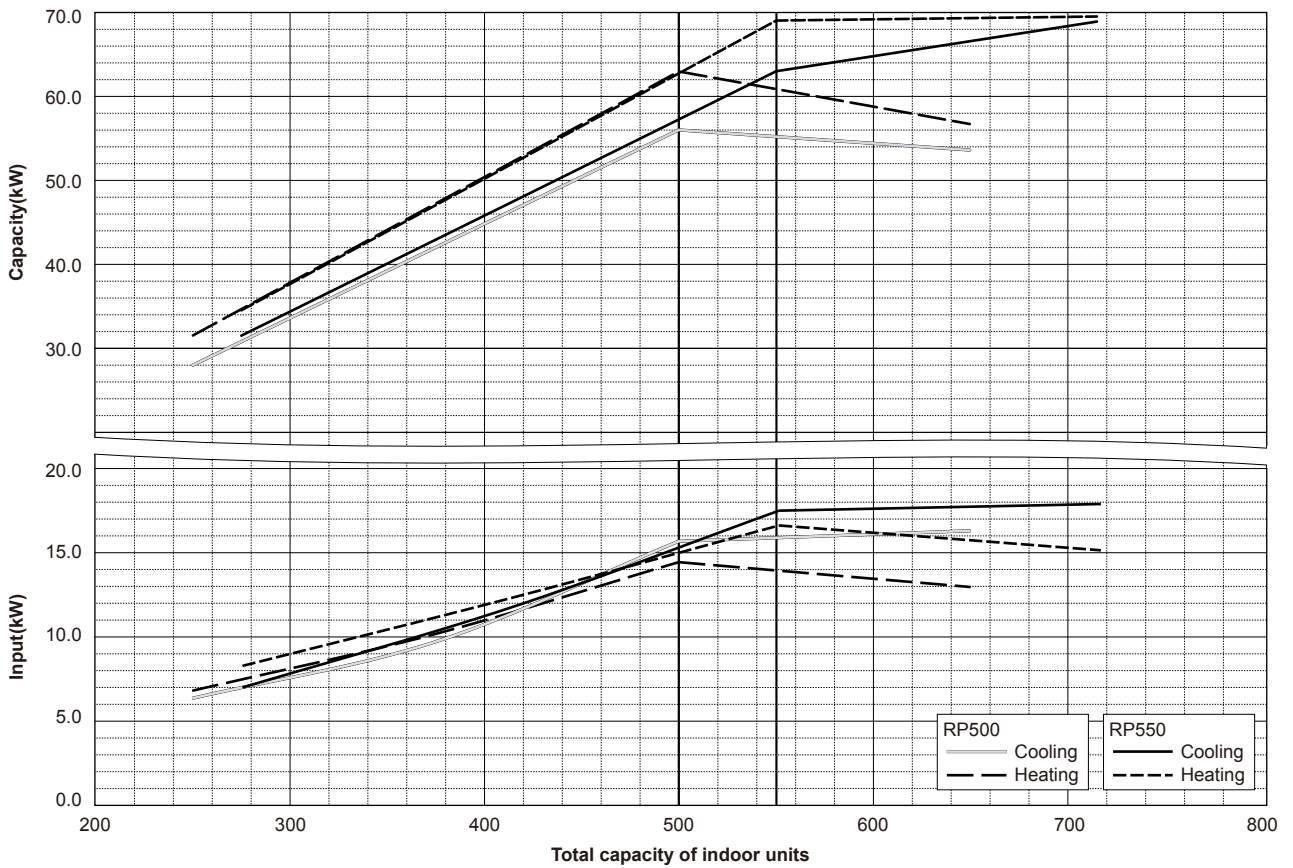
PUHY-RP500, 550YSJM-B(-BS)
