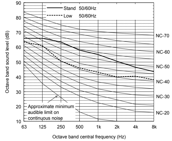
Sound level of PUHY-RP550YSJM-B(-BS)
