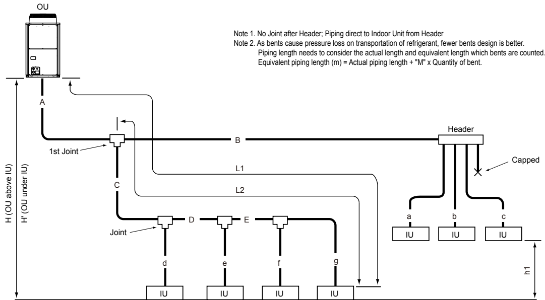
Fig. 3-1-1A Piping scheme
