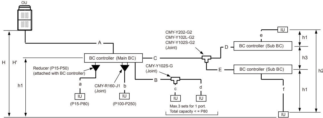
Fig. 3-1-2B Piping scheme
