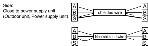
Figure A. Non-using wiring
