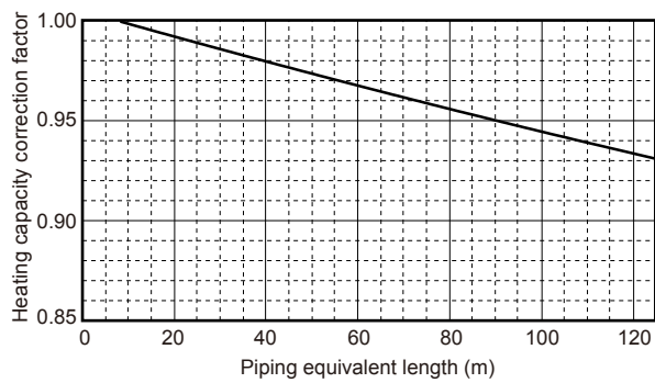
PURY-RP250YJM-B(-BS)
