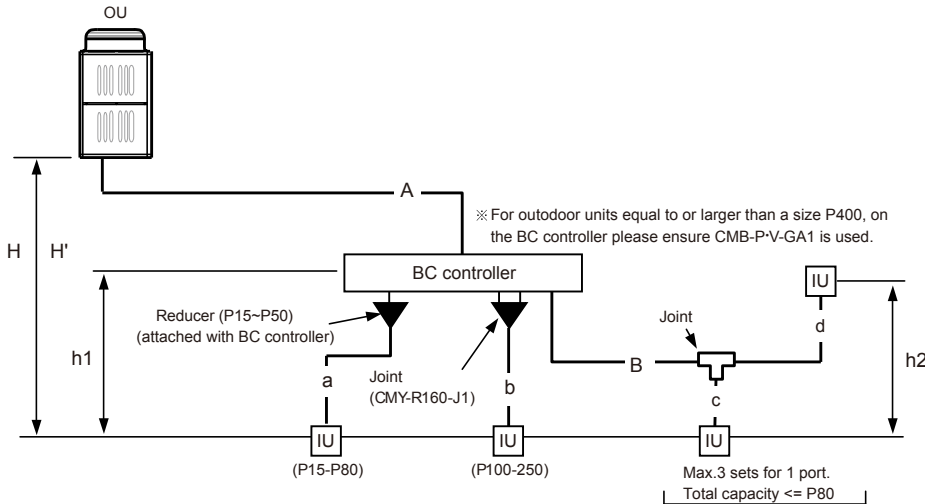
Fig. 3-1-1A Piping scheme
