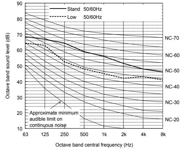
Sound level of PUHY-RP600YSJM-B(-BS)
