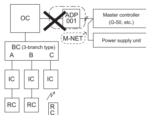
3-3. Connection of M-NET adapter to outdoor unit
