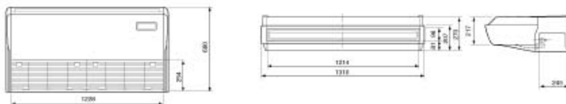
Side View >
