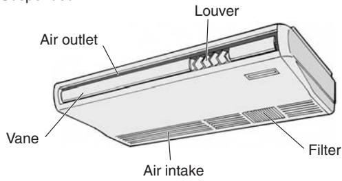
■ PCA-RP-GA/PCH-P-GAH Ceiling Suspended
