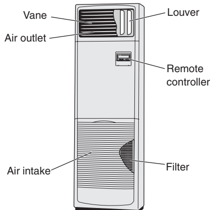
■ PSA-RP-GA/PSH-P-GAH Floor Standing
