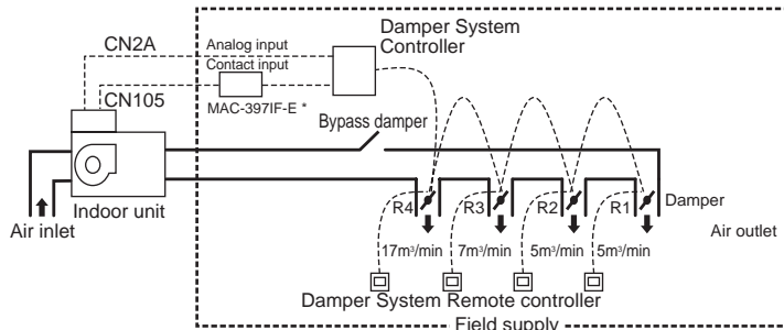
[Fig.1-4-1] Example of duct system
