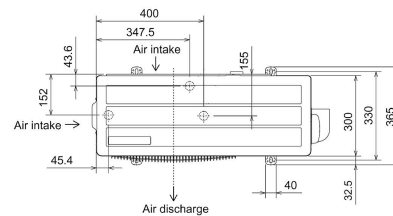
Upper View >
