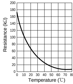
Fin temperature thermistor (RT65) Defrost temperature thermistor (RT62) Outdoor heat exchanger temperature thermistor (RT68)
