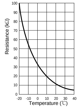
Fin temperature thermistor (RT65) Defrost temperature thermistor (RT62) Outdoor heat exchanger temperature thermistor (RT68)
